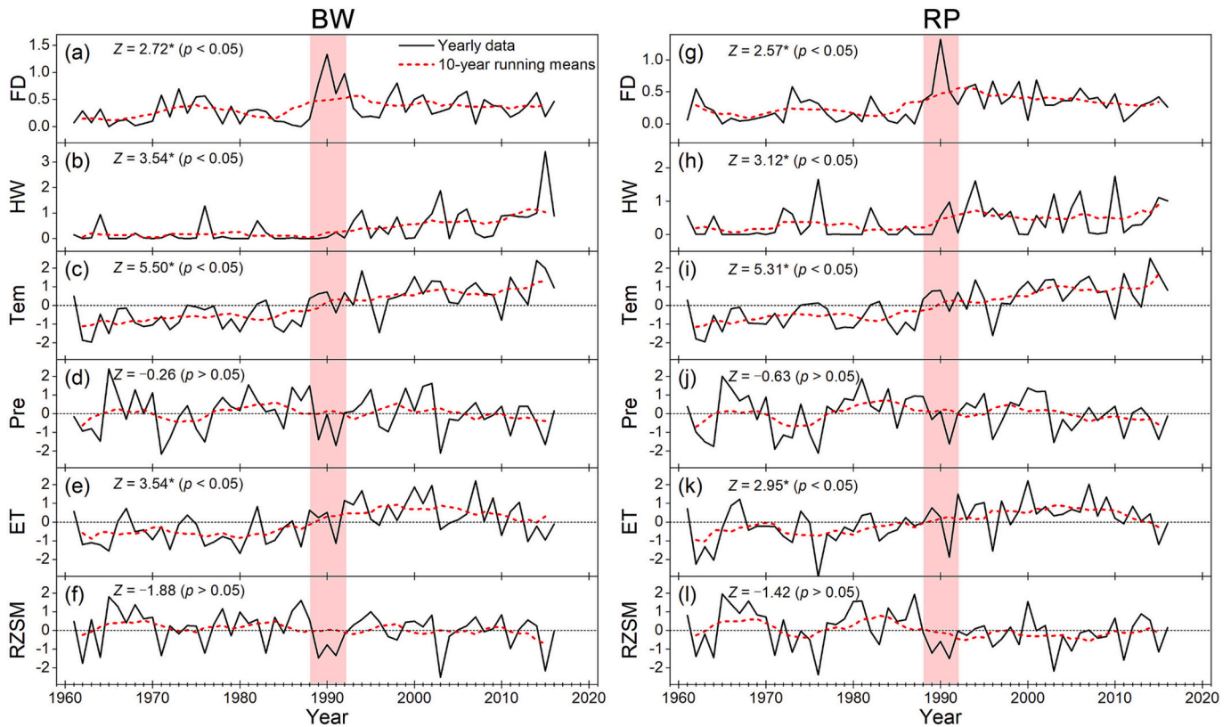
Fig. 6. Regional average annual and decadal variations in flash and heat wave events and their component variables across the study area. (a) and (g) The number of flash drought (FD) events per year; (b) and (h) the number of heat waves (HW) events per year; (c) and (i) temperature (Tem) anomaly, (d) and (j) precipitation (Pre) anomaly, (e) and (k) evapotranspiration (ET) anomaly, and (f) and (l) root zone soil moisture (RZSM) anomaly. Except for the number of flash drought and heat wave events ((a), (b), (g), and (h)), the component variables ((c)–(f) and (i)–(l)) are standardized before being averaged to facilitate the comparison. The Z values are the Mann-Kendall test results; Z values reaching the 0.05 significance level ( p < 0.05 ) are marked with an asterisk. The pink shaded area covers the year (i.e., 1990) when the peak of the flash drought numbers appeared and its adjacent years.
