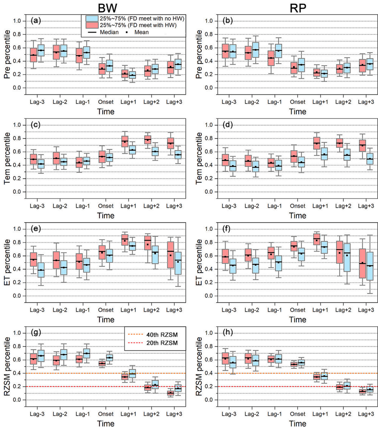
Fig. 11. Percentile changes in the hydro-meteorological variables (precipitation (Pre), Temperature (Tem), Evapotranspiration (ET), and root zone soil moisture (RZSM)) of the two types of flash drought events (i.e., a flash drought (FD) meets with or without a heat wave (HW) event) in adjacent pentads of flash drought onset. “Lag-1” denotes 1 pentad prior to the onset time, while “Lag+1” denotes 1 pentad after the onset time.
