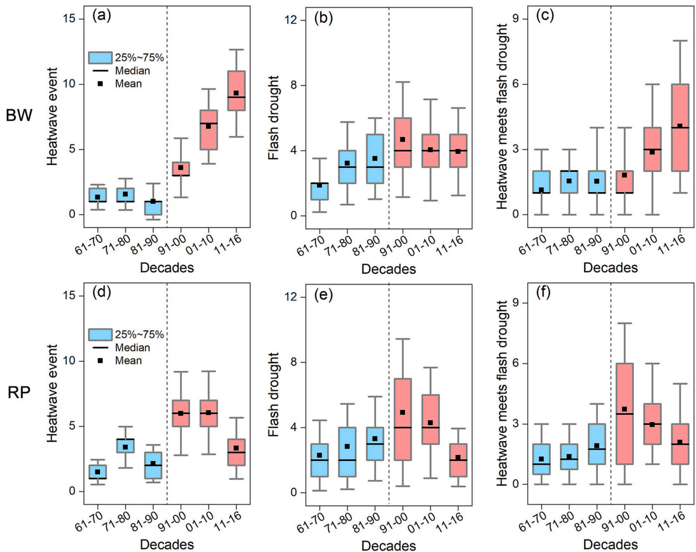
Fig. 8. Number of heat waves ((a) and (d)) and flash droughts ((b) and (e)), and the coincidence of these two events ((c) and (f)) during the past six decades for the Baden-Württemberg (BW) and Rhineland-Palatinate (RP) states.
